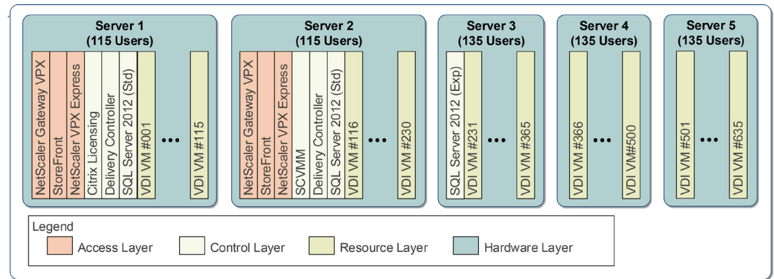
Figure 3: Virtual machine server allocation
