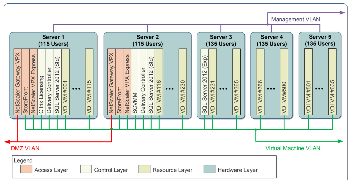
Figure 4: Networking architecture
