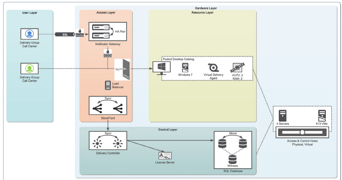
Figure 1: Conceptual architecture
